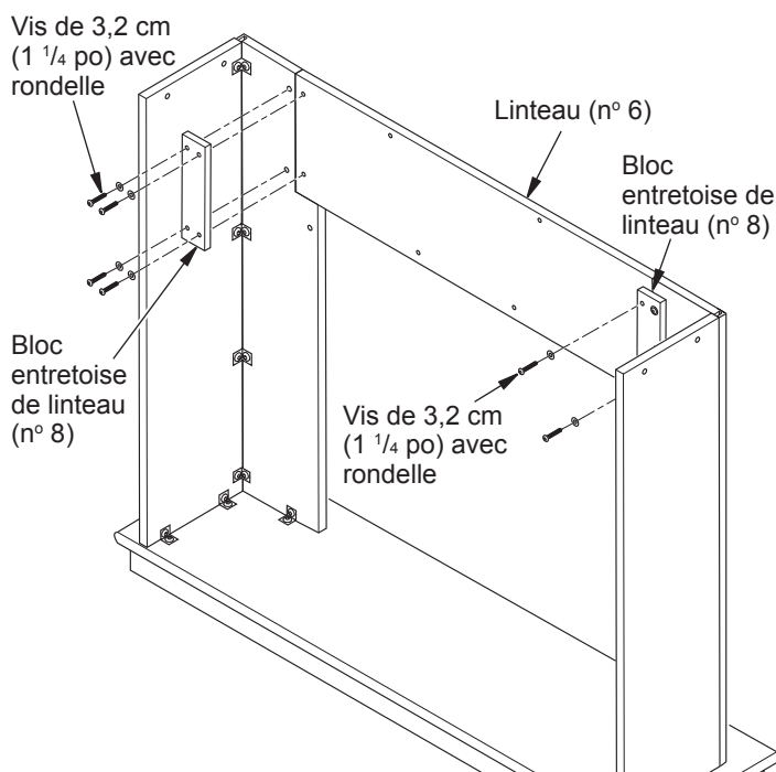
Figure 3 - Pose du linteau
